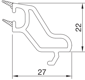
PDR2060BY.0001 24 MM DEKORATİF CAM ÇİTASI 24 MM DECORATIVE GLAZING BEAD
