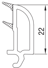
PSC9660BY.0001 40 MM CAM ÇİTASI 40 MM GLAZING BEAD
