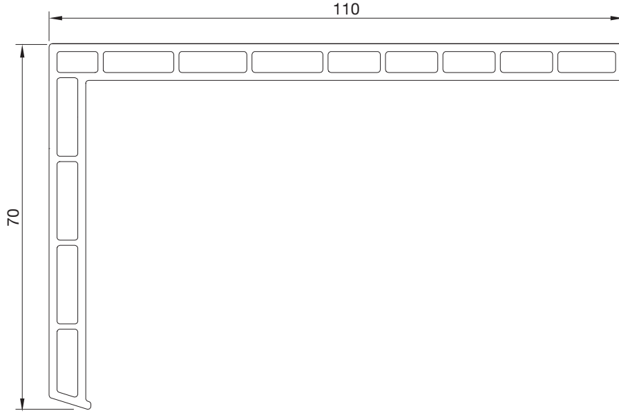
PTS3560BY.0003 PERVAZ PROFİLİ CASING PROFILE
