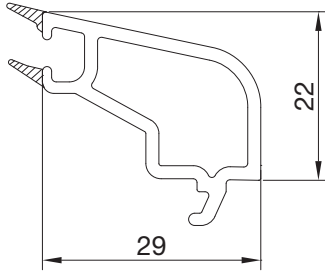
PDR1760BY.0003 20 MM CAM ÇİTASI 20 MM GLAZING BEAD
