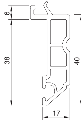
PTS3660BY.0003 DEKORATİF PERVAZ PROFİLİ DECORATIVE CASING PROFILE
