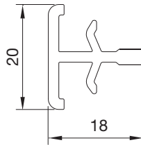
PTS3160BY.0003 İNCE BAĞ PROFİLİ COUPLING PROFILE
