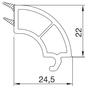
PSC1960BY.0001 24 MM CAM ÇİTASI 24 MM GLAZING BEAD
