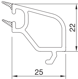
PDR1960BY.0001 24 MM CAM ÇİTASI 24 MM GLAZING BEAD
